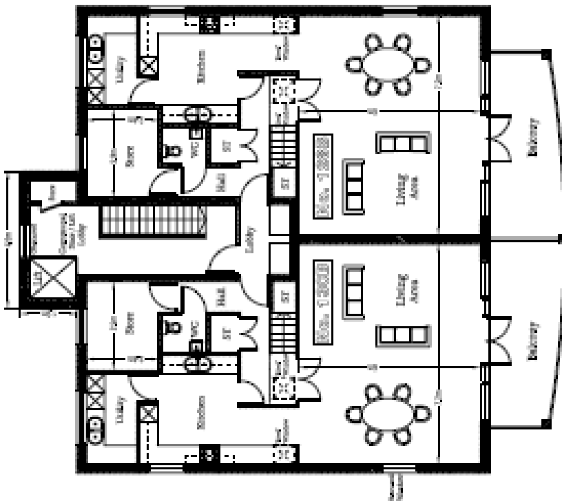
Proposed Second Floor Plan @ 1:100
